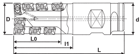
Fig. 5 (coolant thru)
